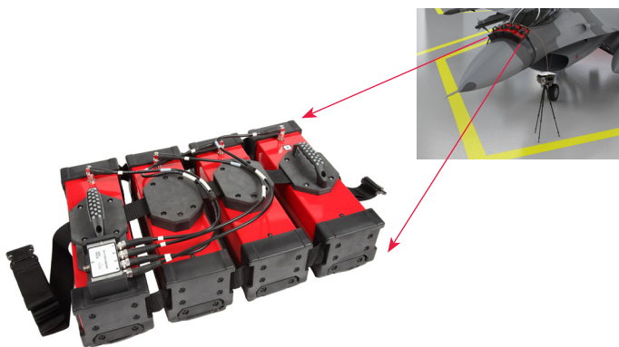
Interrogator Coupler
